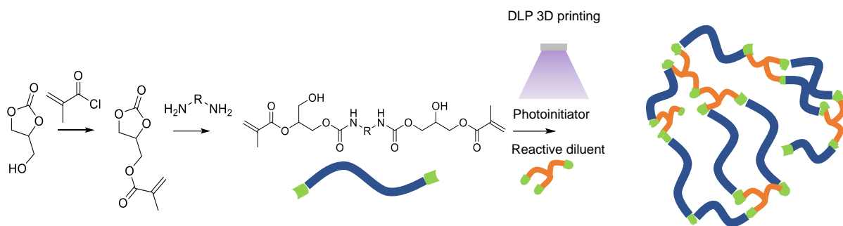
Synthesis of polyhydroxyurethanes for 3D printing by vat photopolymerization
