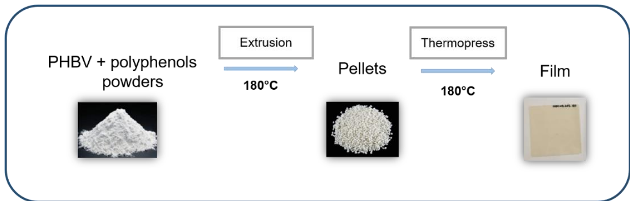
Processing procedure to produce PHBV/polyphenols blend films from powders
